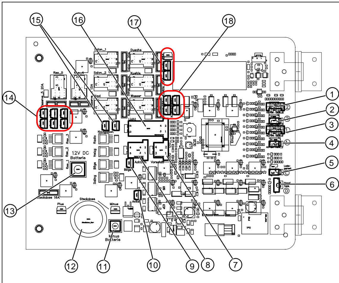
Fig. 7 Rear view of the panel 301 - terminal assignment
